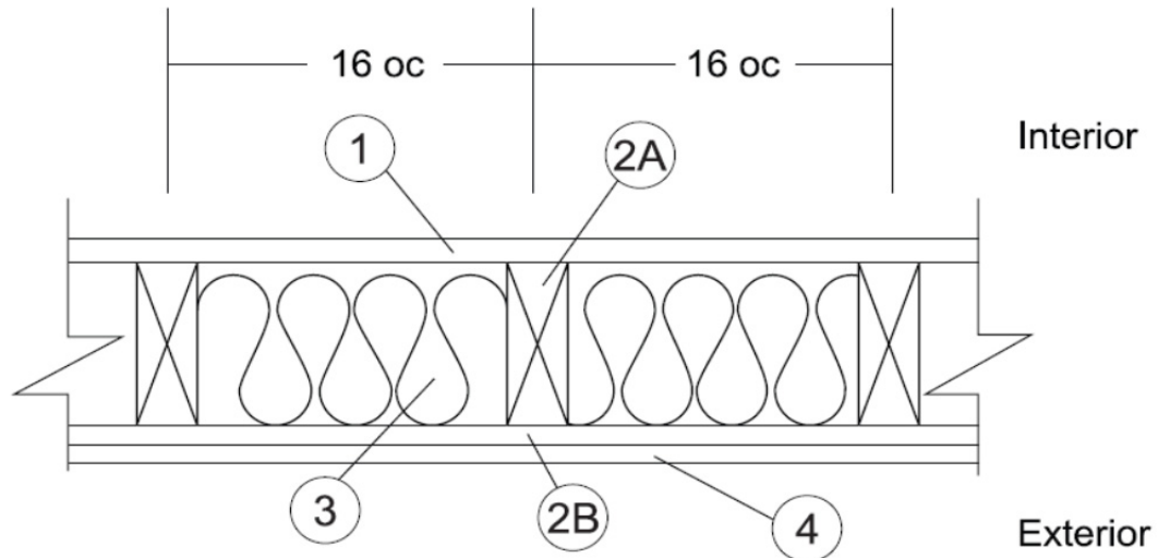
FIGURE 2—ONE-HOUR FIRE RESISTANCE ASSEMBLY
